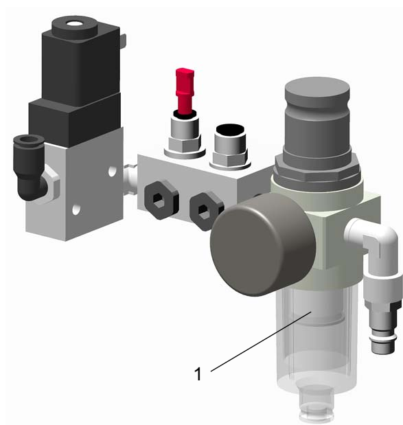
OptiFlex 2 Q - Pneumatic group
